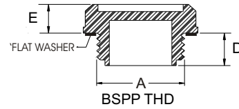
BSPP THD
