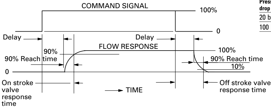
Step response definition of terms
