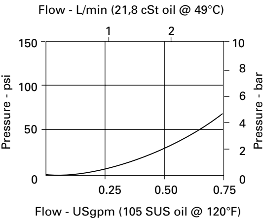
Pressure override, de-energized
